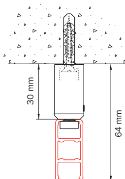
ceiling mounting 4100 with suspension hanger 4254
