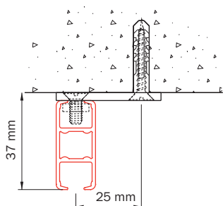
ceiling mounting 4100 with ceiling bracket 4135
