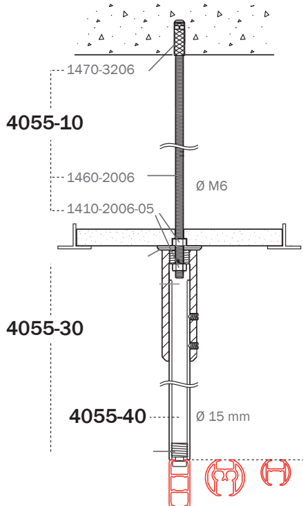
- ceiling mounting 4100, 5100 or 4200: threaded rod set 4055-10, suspension hanger tube 4055-40 and with mounting set 4055-30.
