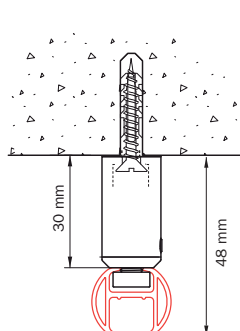
ceiling mounting 4200 with suspension hanger 4254
