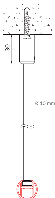
ceiling mounting with 4255
