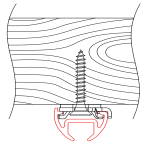
ceiling fixing (profile 2600) with clamp 2650, washer 2649 and special screw 2614
