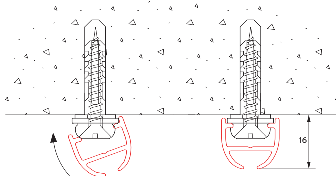
ceiling fixing (profile 2500) with button clip 2254 and washer 2649
