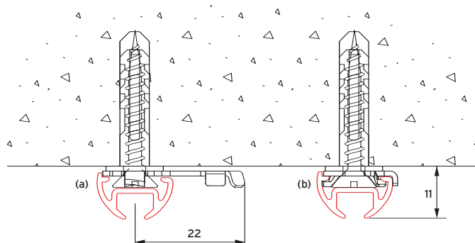
ceiling fixing (profile 2600) with clamp 2650 (incl. washer 2649).
